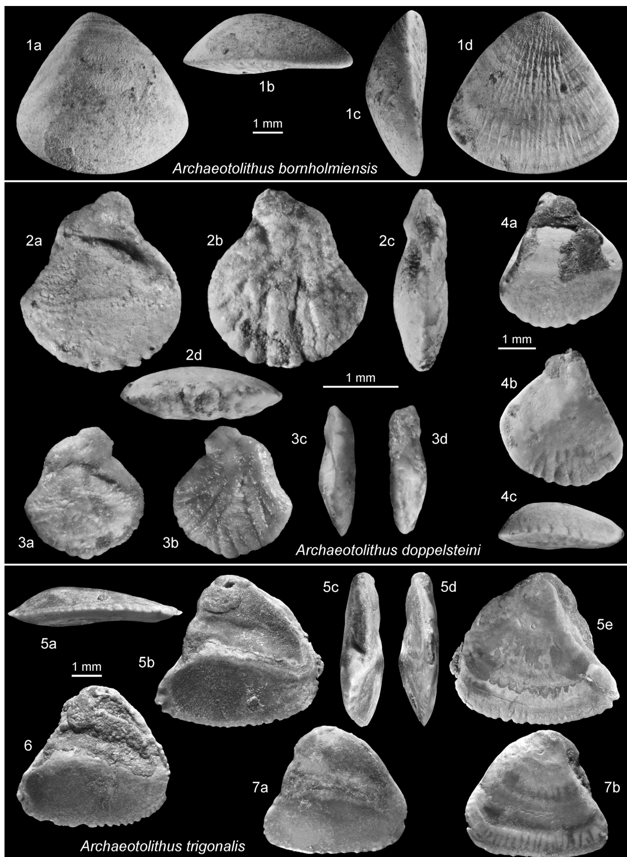
Plate 4. Otoliths of Archaeotolithus . fig. 1: Archaeotolithus bornholmiensis (Malling & Grønwall, 1909), from the late Pliensbachian of Buttenheim, holotype SNSB-BSPG 2022 IV 7, EPH horizon. figs 2–4: Archaeotolithus doppelsteini sp. nov., from the late Pliensbachian of Buttenheim, EPH horizon; 2: holotype SNSB-BSPG 2022 IV 8; 3–4: paratypes SNSB-BSPG 2022 IV 9. figs 5–7: Archaeotolithus trigonalis Stolley, 1912, from the late Pliensbachian of Buttenheim, EPH horizon, figured specimens SNSB-BSPG 2022 IV 12.
