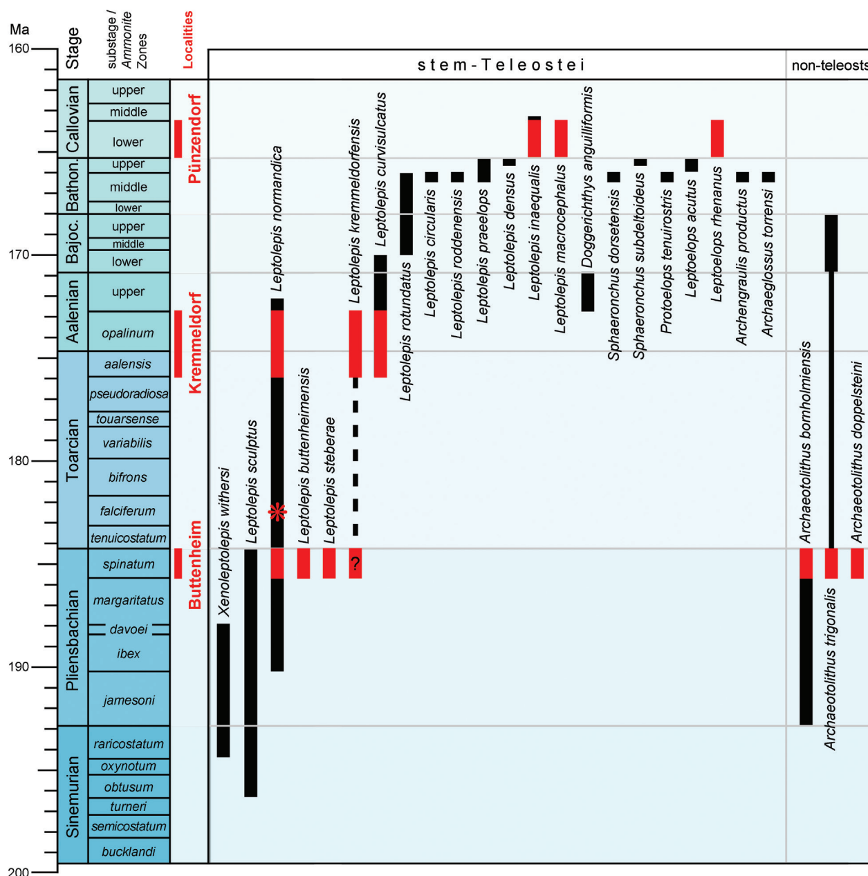
Figure 4. Stratigraphic chart depicting ranges of Early to Middle Jurassic otolith-based fish species. Red bars reflect ranges of localities from which otoliths have been studied for this article. The red asterisk indicates the stratigraphic position of the fishes with otoliths in situ described by Delsate (1997). Chronostratigraphy and ammonite zonation after Gradstein et al. (2020).
