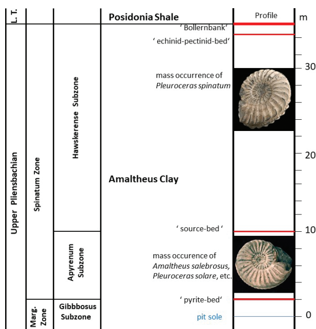
Figure 2. Stratigraphic scheme for the Buttenheim clay pit after Keupp (2021a). Otolith bearing sampled intervals are the ‘echinid-pectinid-bed’ (EPH), the ‘source-bed’ (Quellhorizont) and the Apyrenum subzone.
